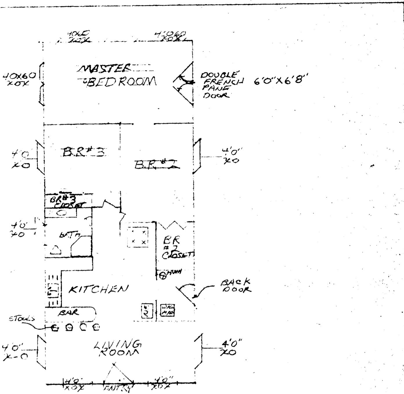
FLOOR PLAN SCALE = 1/8" = 1'00"
