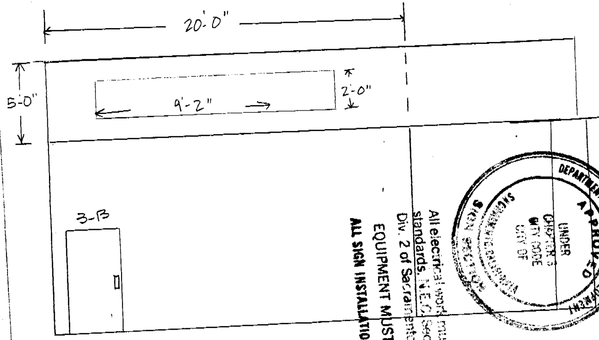
FRONT ELEVATION
