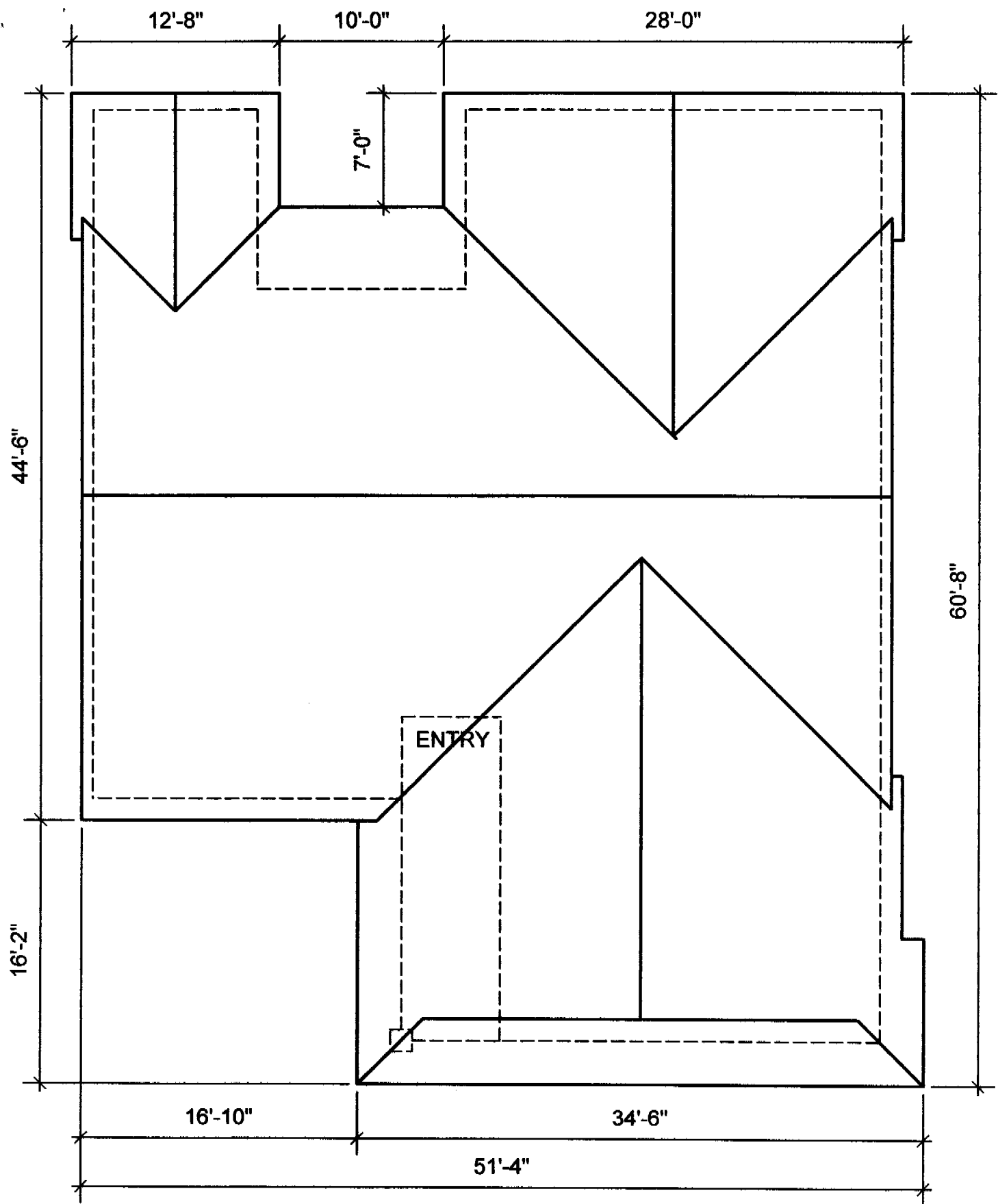
10 DAKOTA COURT SCHEMATIC ROOF PLAN (DIMENSIONS ARE APPROXIMATED)
