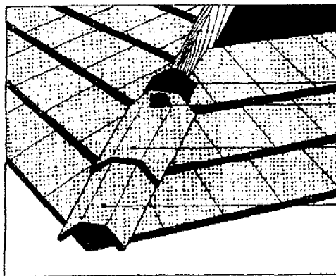
FIGURE 2—TYPICAL INSTALLATION DETAILS
