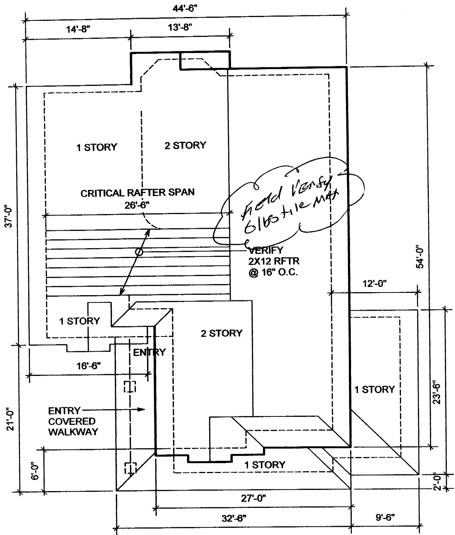
125 PINEDALE AVENUE SCHEMATIC ROOF PLAN (DIMENSIONS ARE APPROXIMATED)
