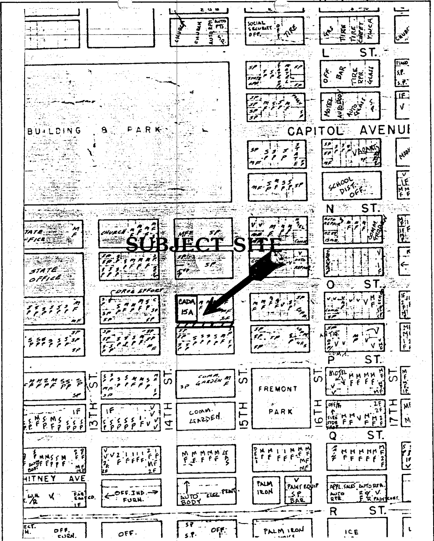
VICINITY MAP
