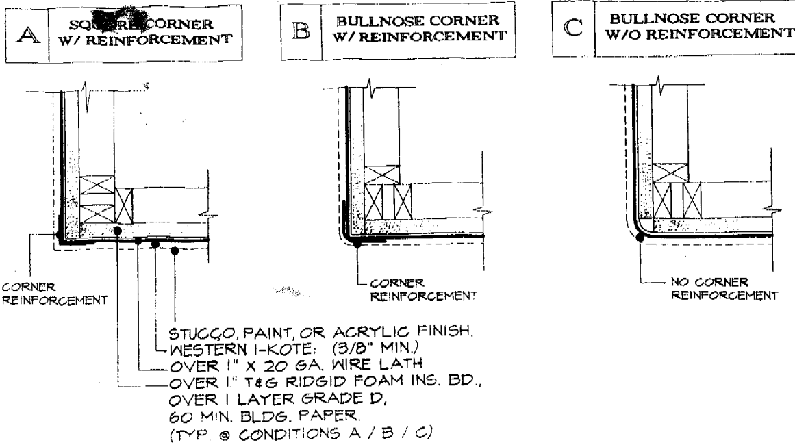
FIGURE 2—TYPICAL INSTALLATION DETAILS—(Continued)
