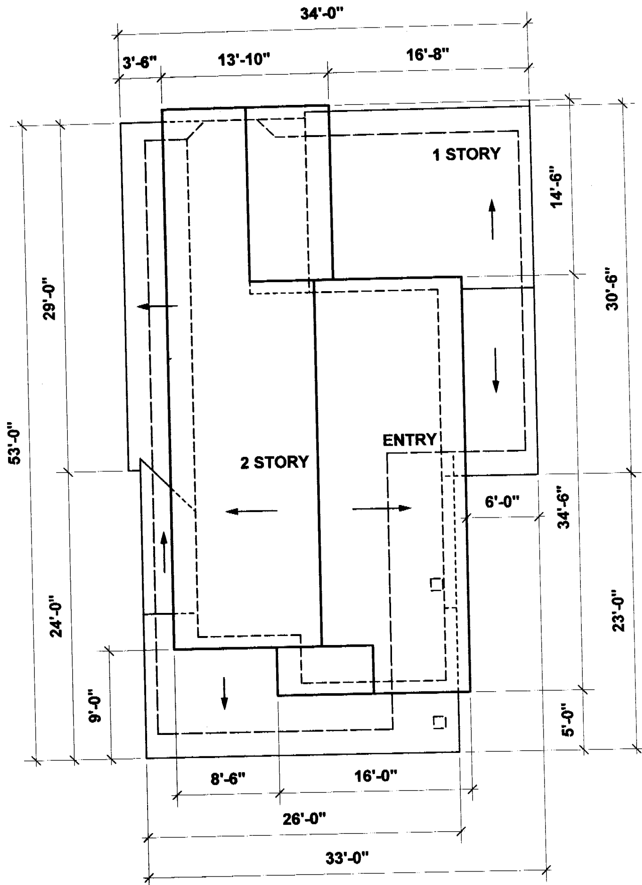
947 RANCHO ROBLE WAY SCHEMATIC ROOF PLAN (DIMENSIONS ARE APPROXIMATED)
