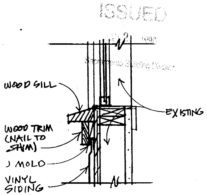
B SILL
