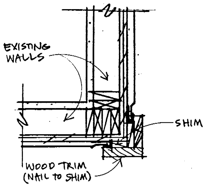
C CORNER
