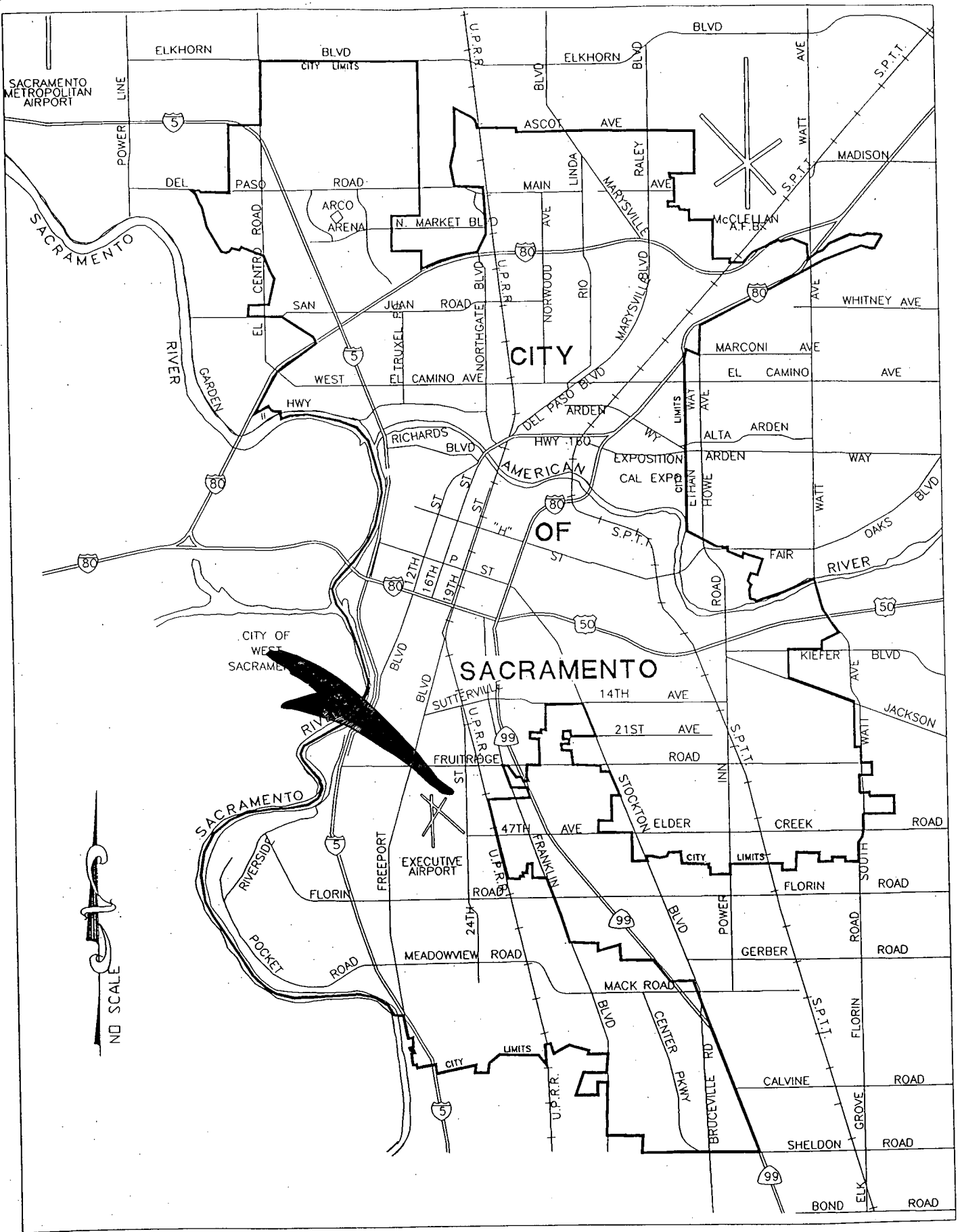
VICINITY MAP
