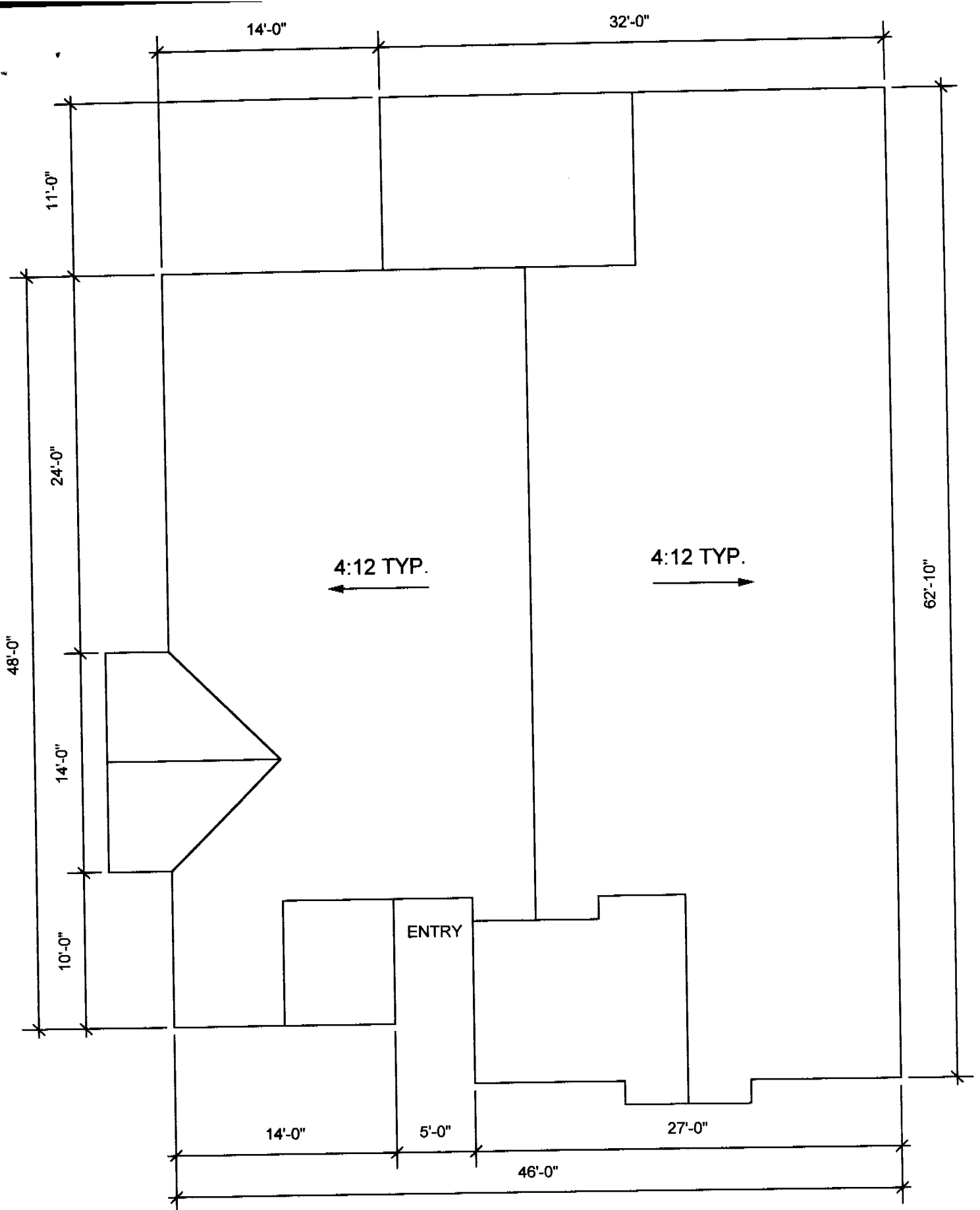
ROOF PLAN 1744 Pebblewood Drive
