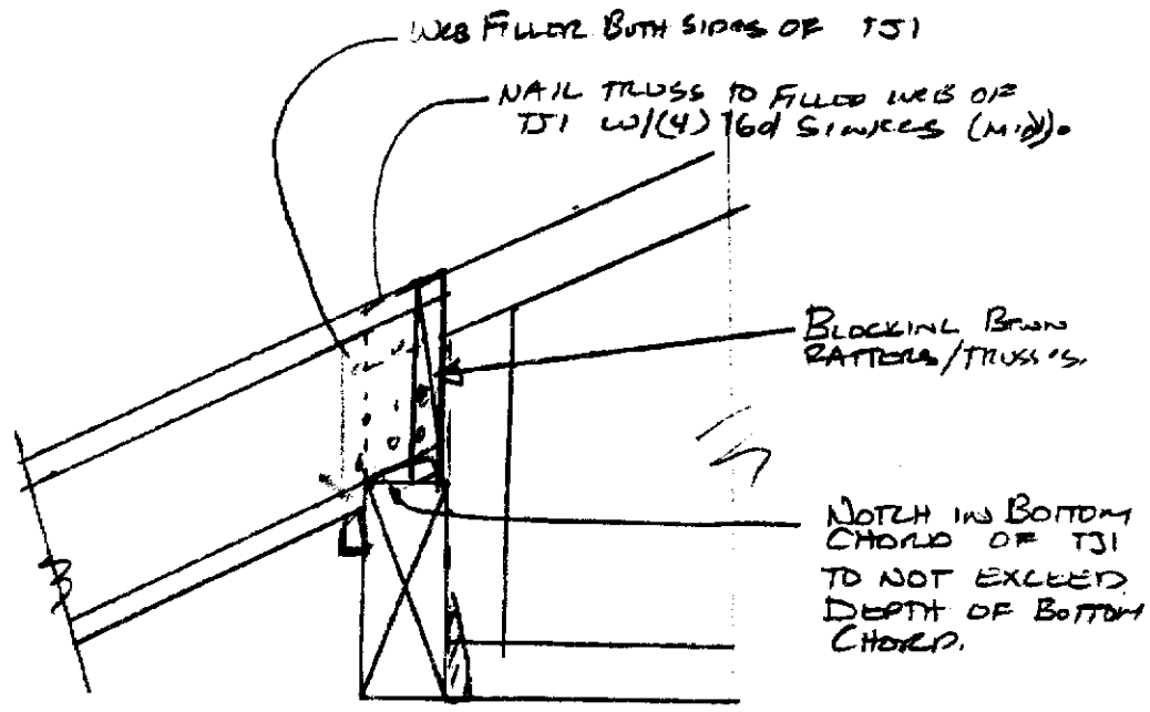
RAFTERS & BEAM OVER STAIRS NTS
