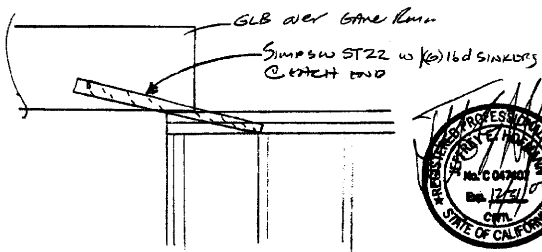
BEAM TO WALL STRAP - GLB over Game Room NTS
