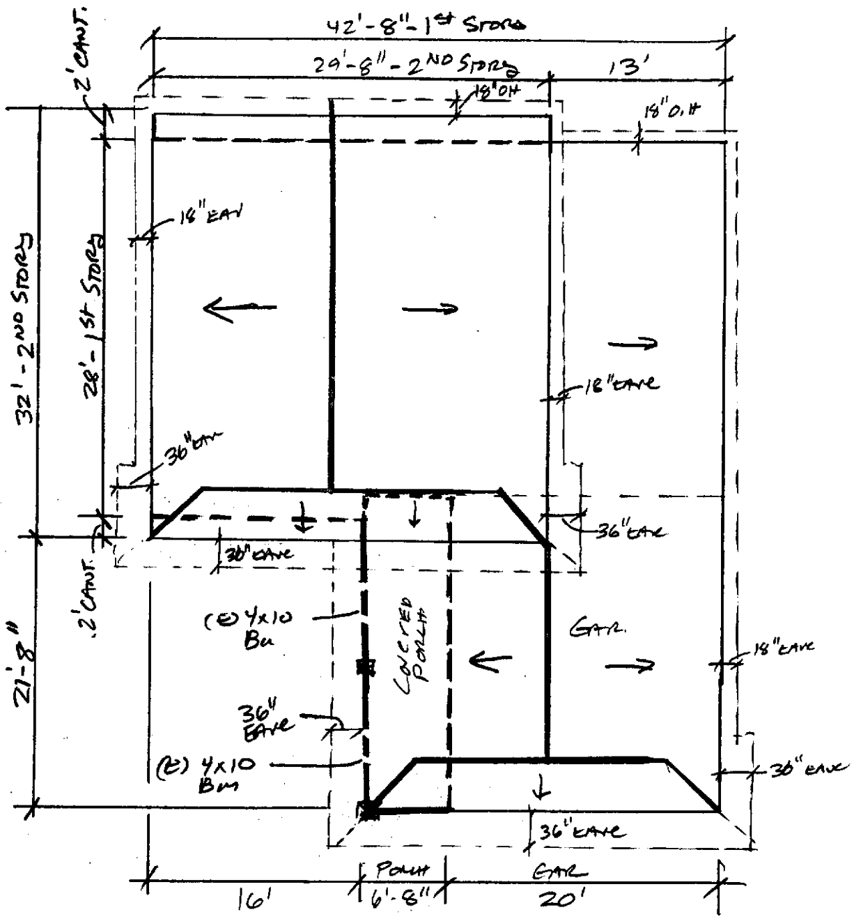
SKETCH - ROOF PLAN SCALE ≈ 1" = 10'
