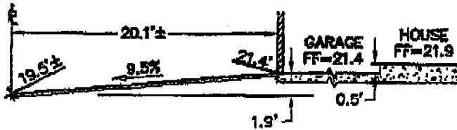
DRIVEWAY CENTERLINE PROFILE (NOT TO SCALE)
