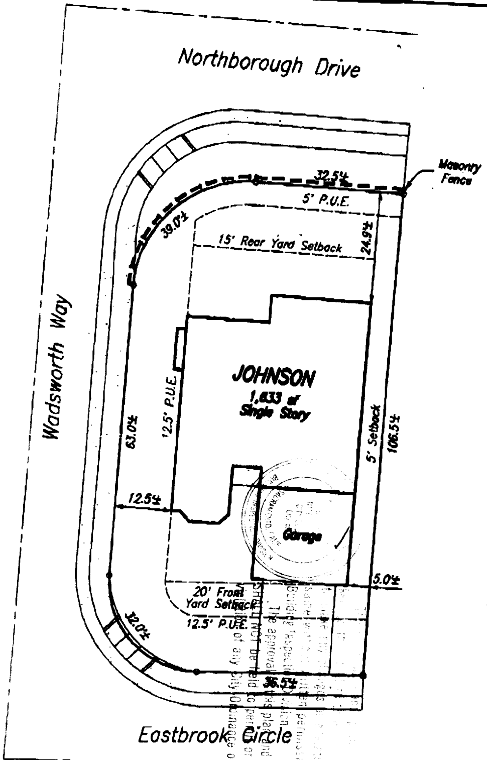
Plot Plan for Lot 17 for Northborough Village J-1 U.S.Home - Northborough - Traditions Series City of Sacramento
