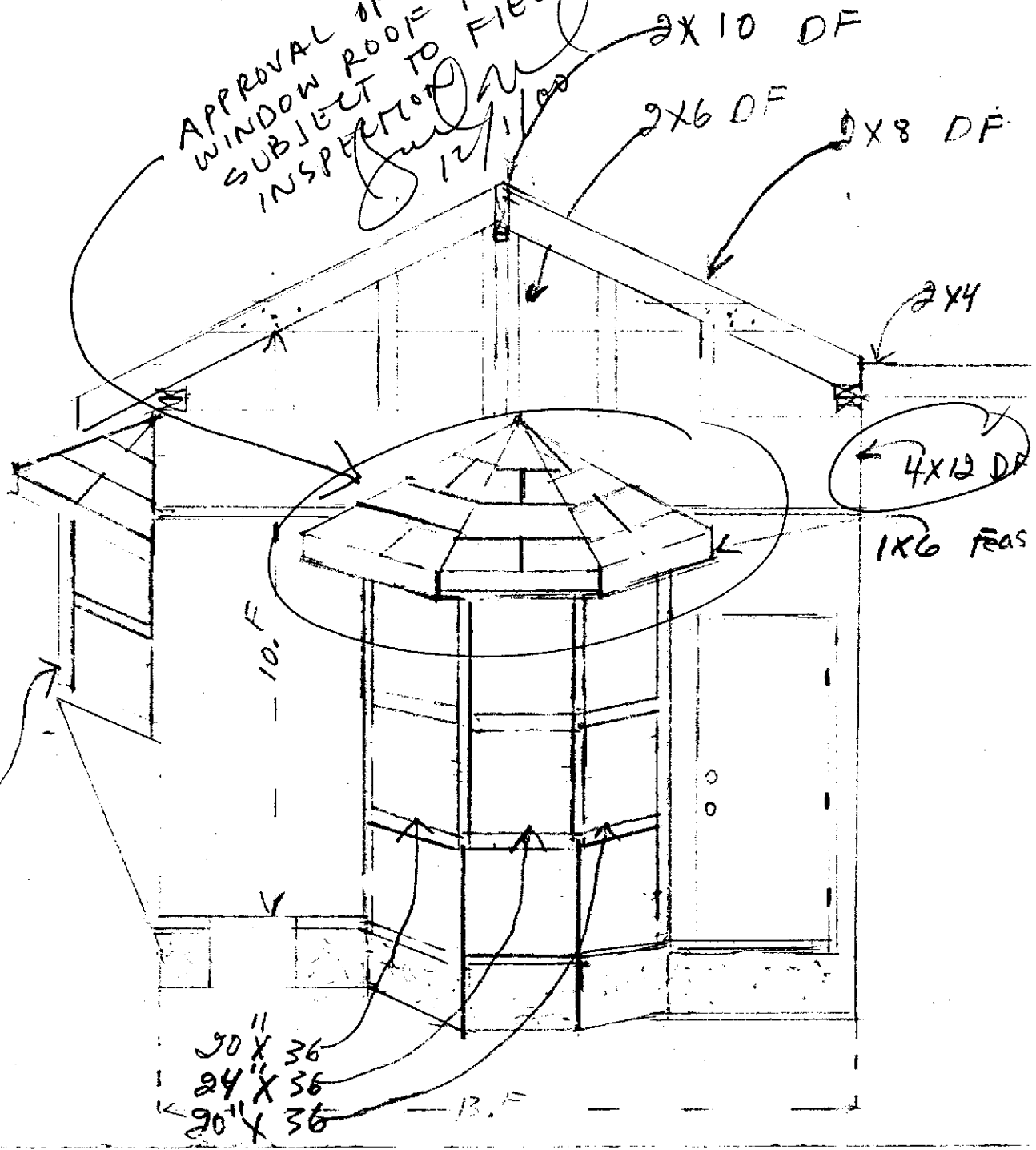
WEST ELEVATION
