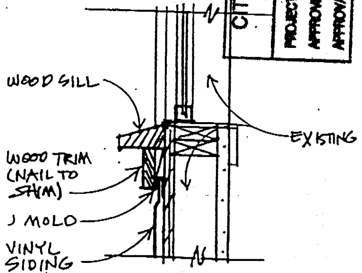
B SILL
