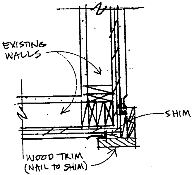
C CORNER
