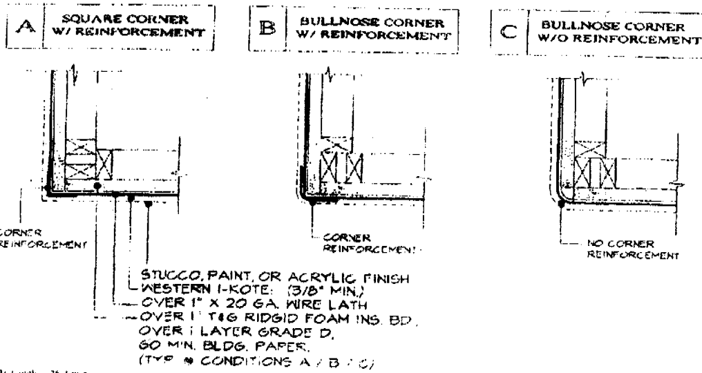
FIGURE 2—TYPICAL INSTALLATION DETAILS—(Continued)
