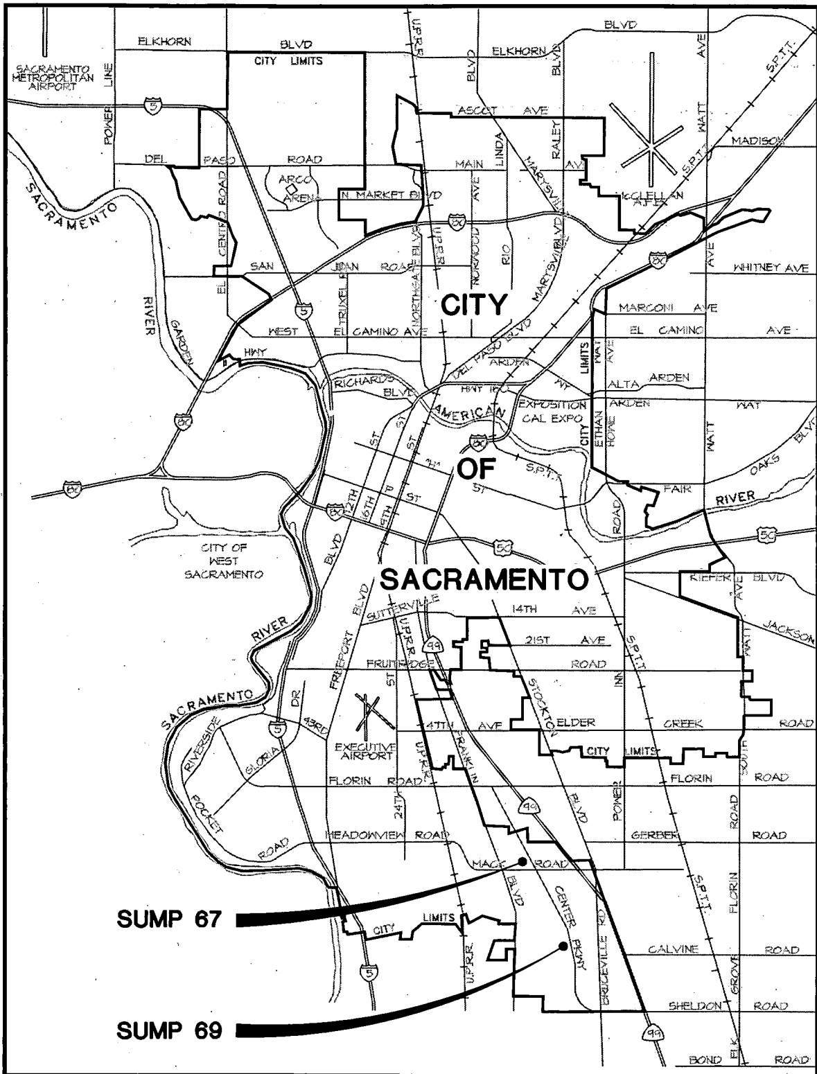
VICINITY MAP
