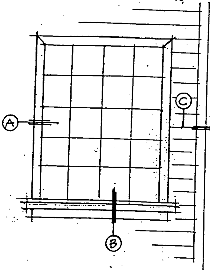
WINDOW ELEVATION
