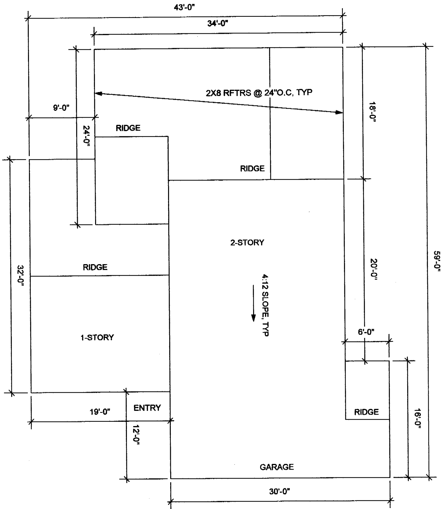
ROOF PLAN 55 TUNDRA WAY
