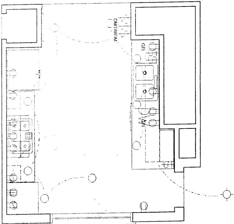
LIFSHER - 1/4"=1'0" - NEW KITCHEN ELECTRICAL PLAN #1
