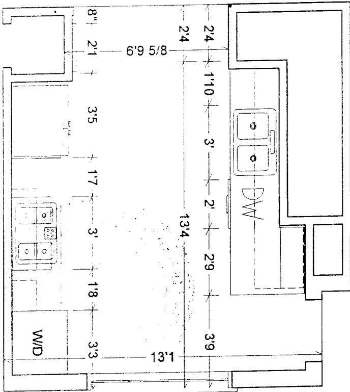
LIFSHER - 1/4"=1'0" - NEW KITCHEN FLOOR PLAN #1
