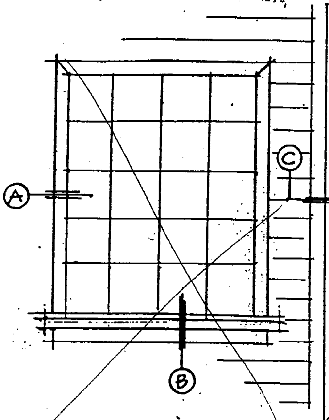
WINDOW ELEVATION
