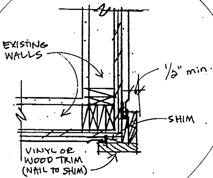
C CORNER
