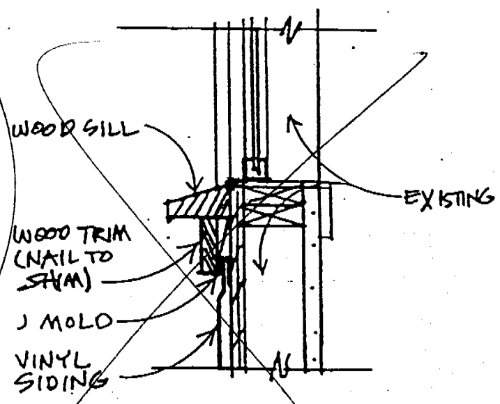
B SILL
