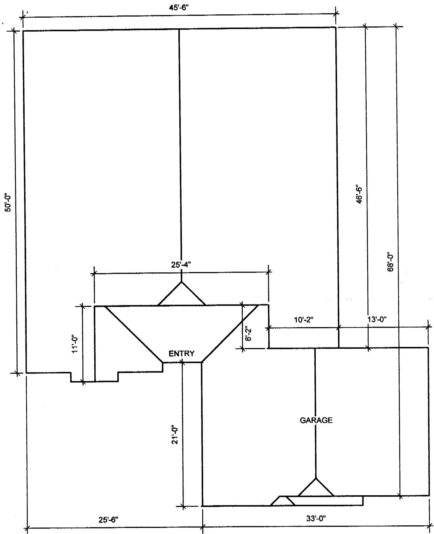
161 PINEDALE AVENUE SCHEMATIC ROOF PLAN (DIMENSIONS ARE APPROXIMATED)
