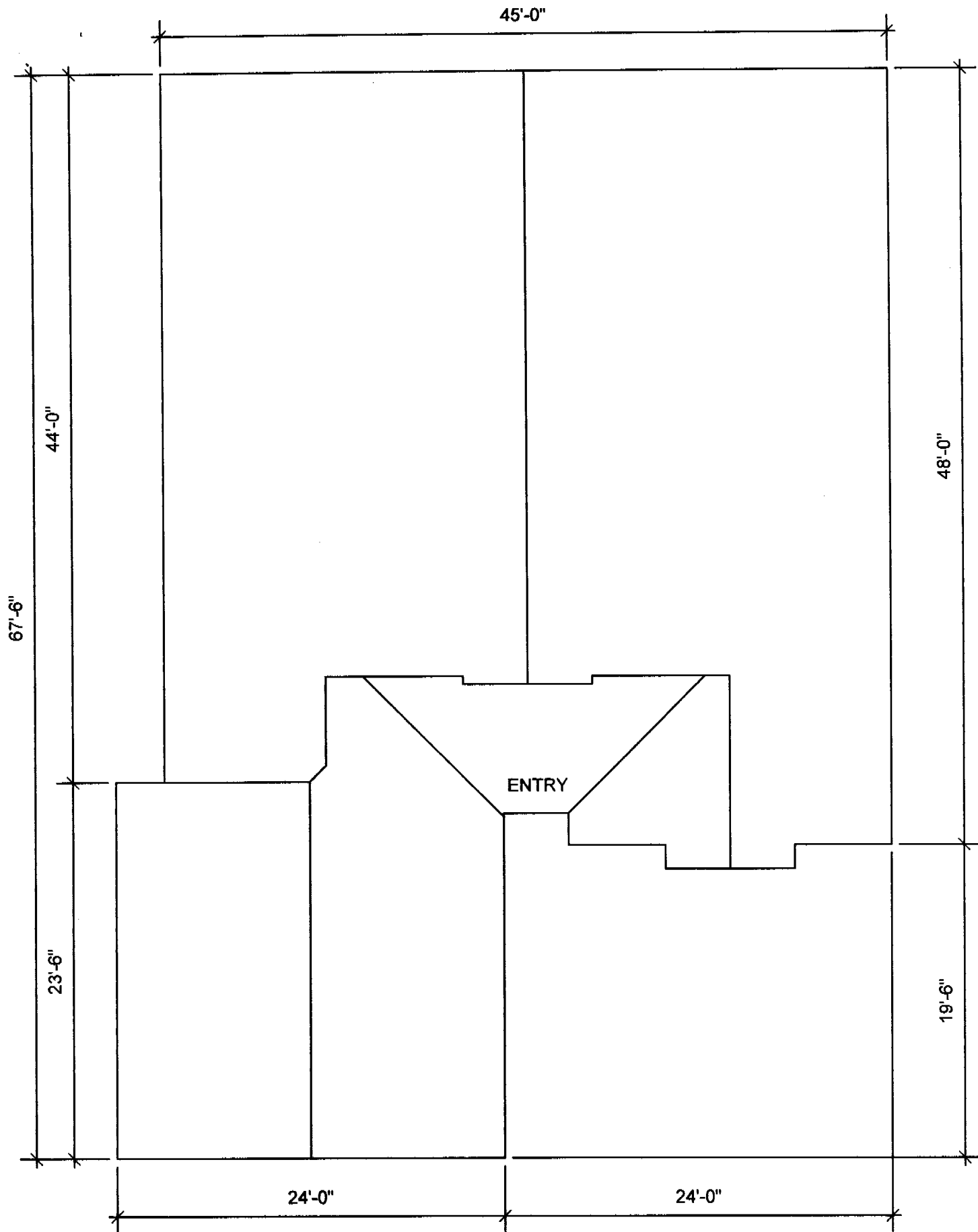
106 PINEDALE AVENUE SCHEMATIC ROOF PLAN (DIMENSIONS ARE APPROXIMATED)
