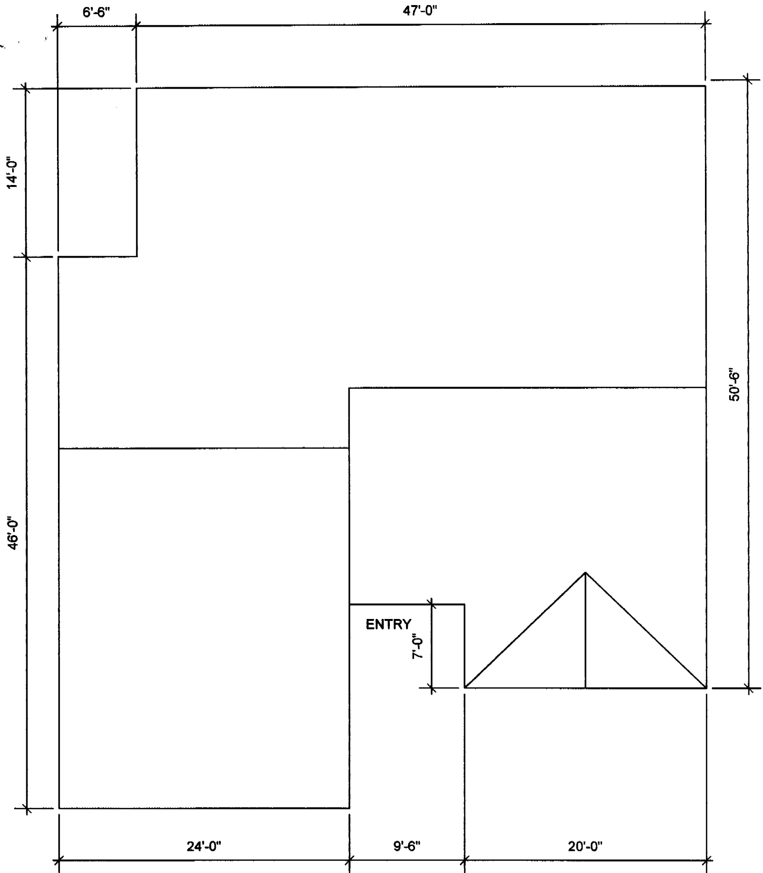
3154 ASUNA WAY SCHEMATIC ROOF PLAN (DIMENSIONS ARE APPROXIMATE)
