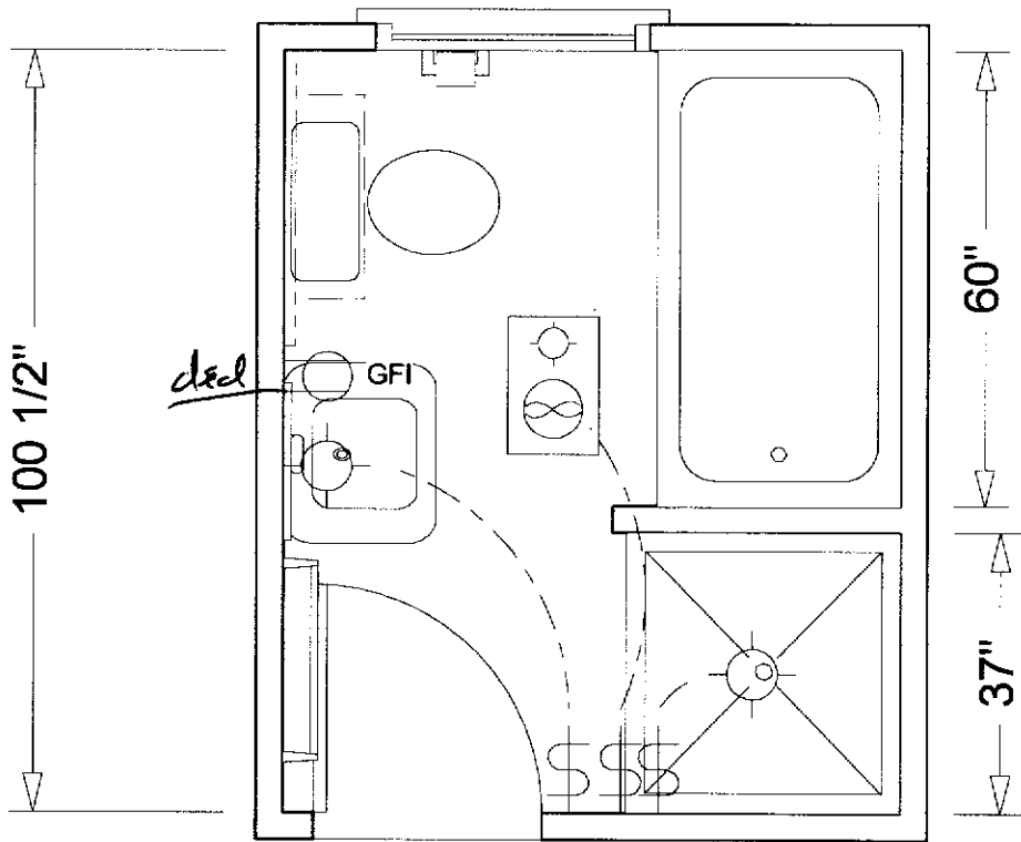
Anne Pings New Bath Electrical Plan
