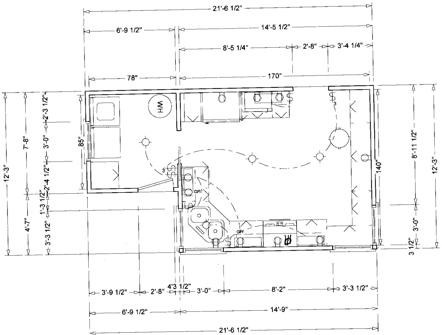
Anne Pings Electrical Plan
