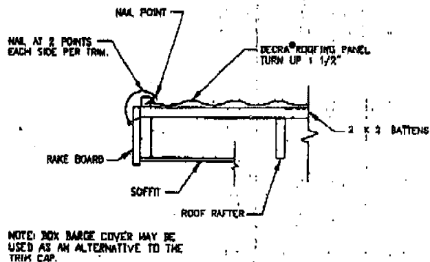
RAKE DETAIL WITH PANEL TURN UP
