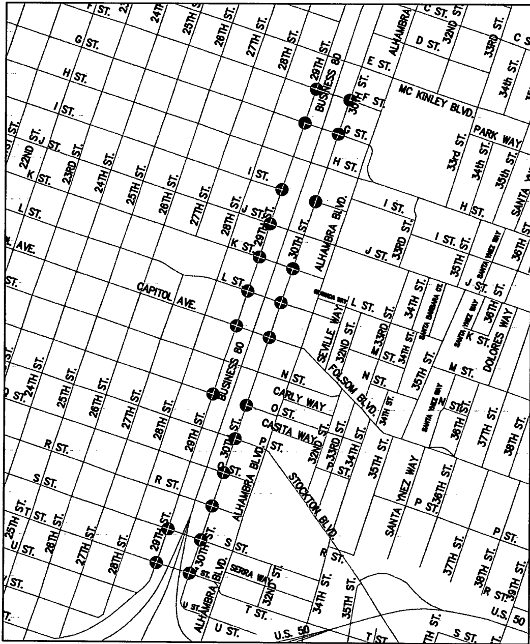
CURB RAMP LOCATIONS 29TH & 30TH STREETS COUNCIL DISTRICT 3&4
