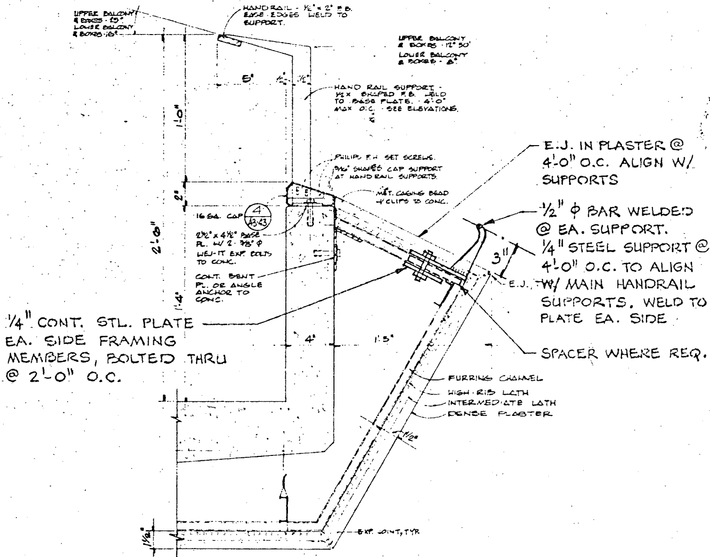
① BALCONY & BOX FRONT RAIL SCALE 1/4\"/>
