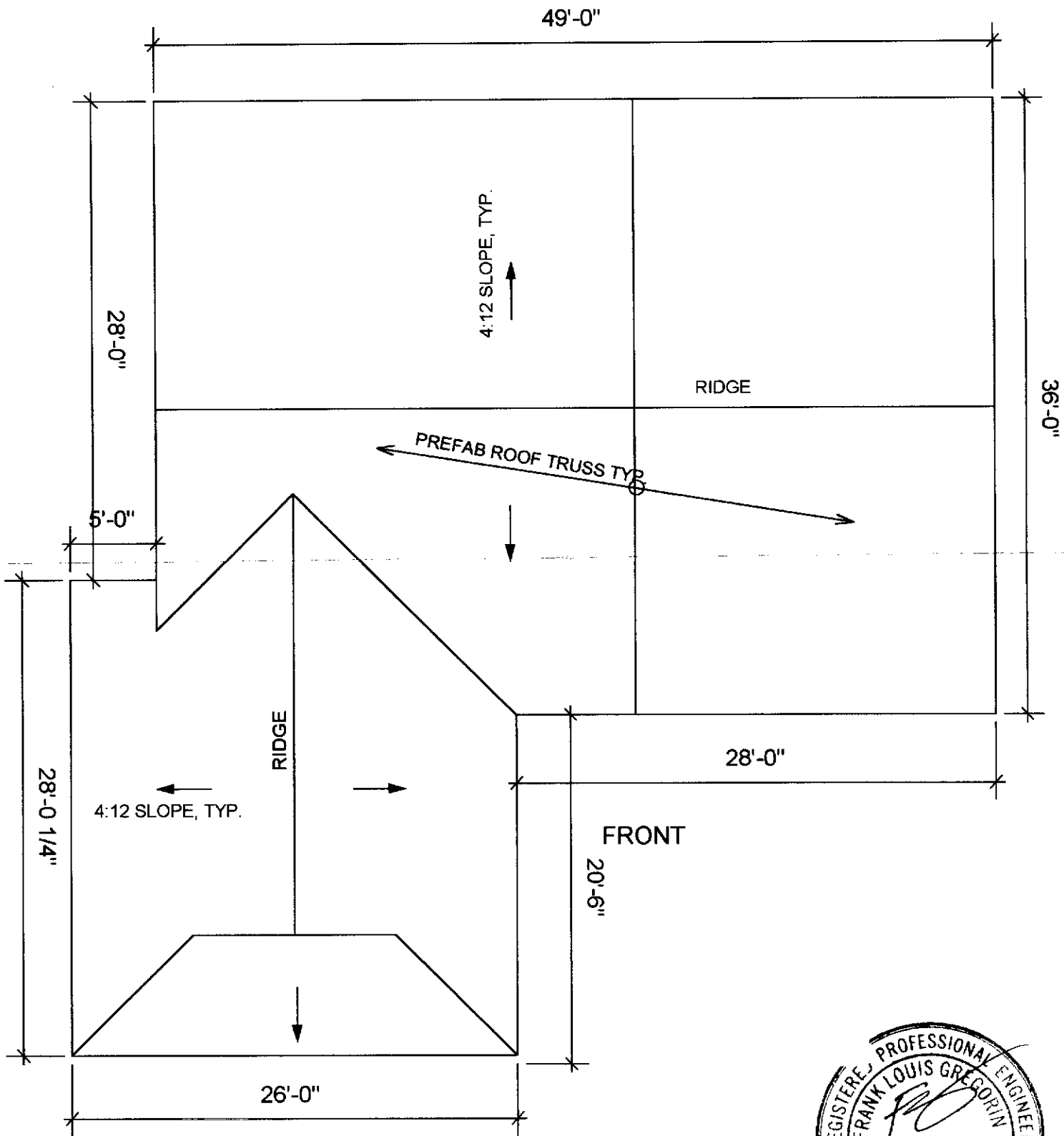
ROOF PLAN 2624 NORBERT WAY
