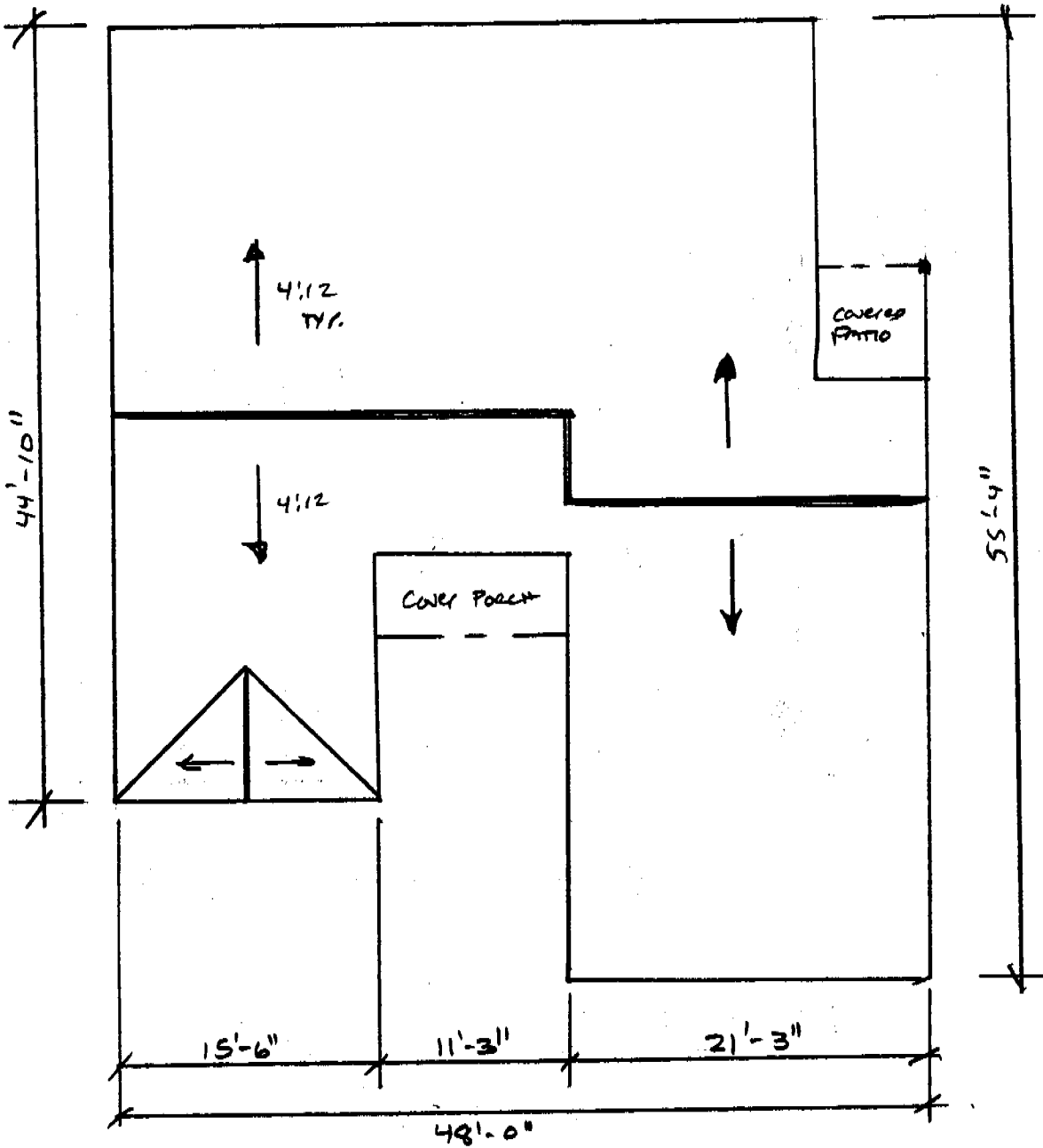
SKETCH OF ROOF PLAN ~ SCALE 1" = 10'
