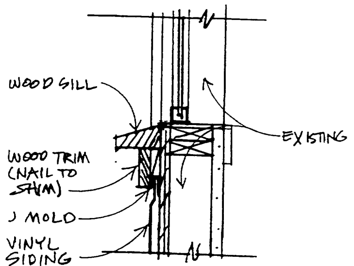
B SILL
