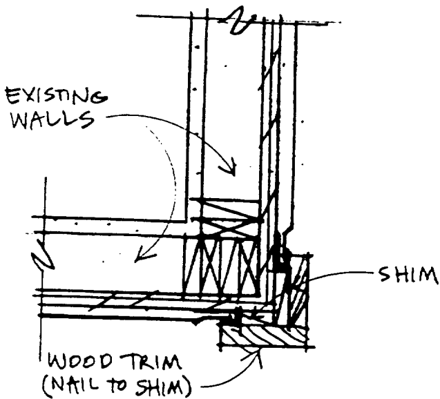
C CORNER
