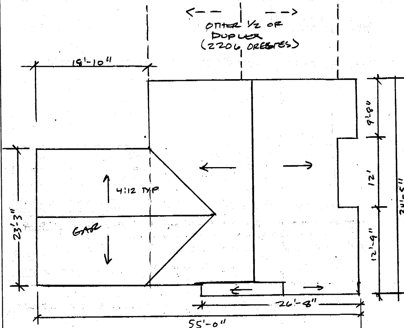
SKETCH OF ROOF (1/2 OF DUPLEX - 2833 AZAVERO)
