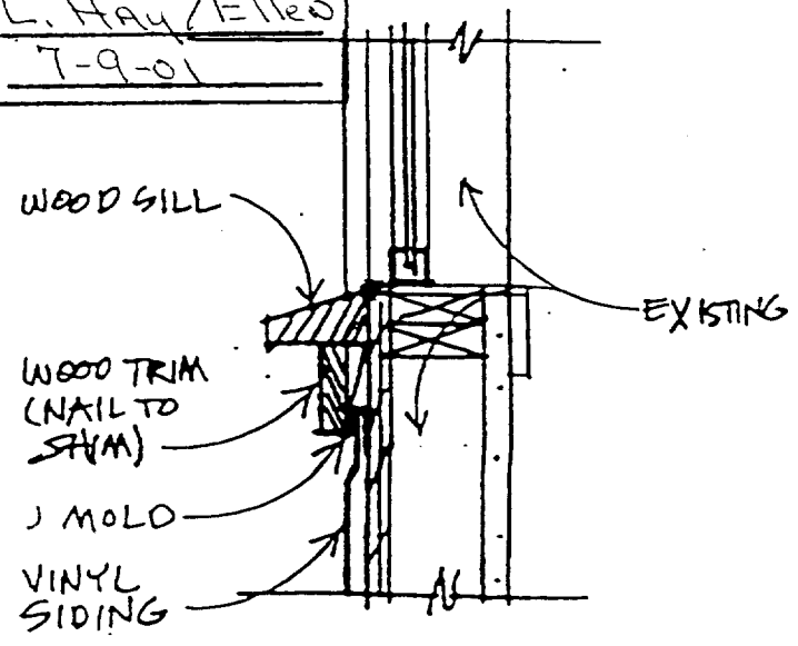
(B) SILL
