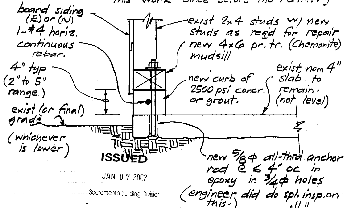
TYP. WALL SECT @ MUDSILL 1 1/2" scale - applies @ N, E, & W sides of Garage
