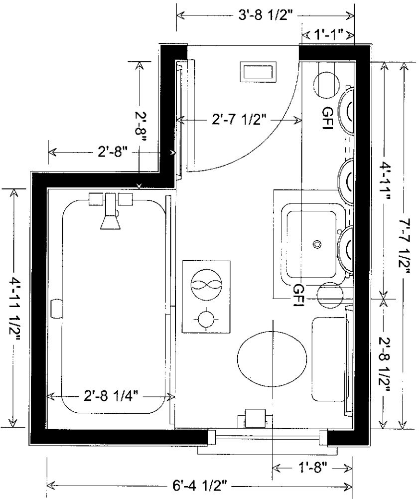
Bonney - New Floor Plan - 1/2"=1'0"
