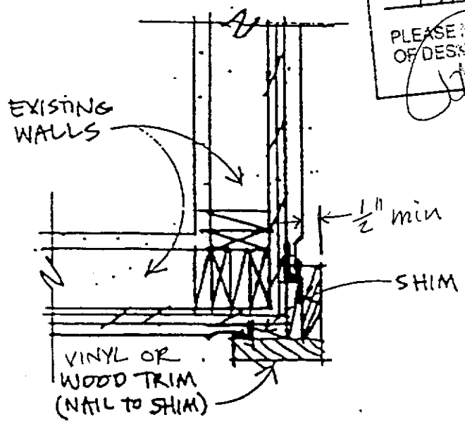
(C) CORNER
