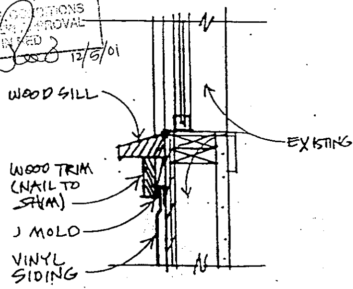
(B) SILL
