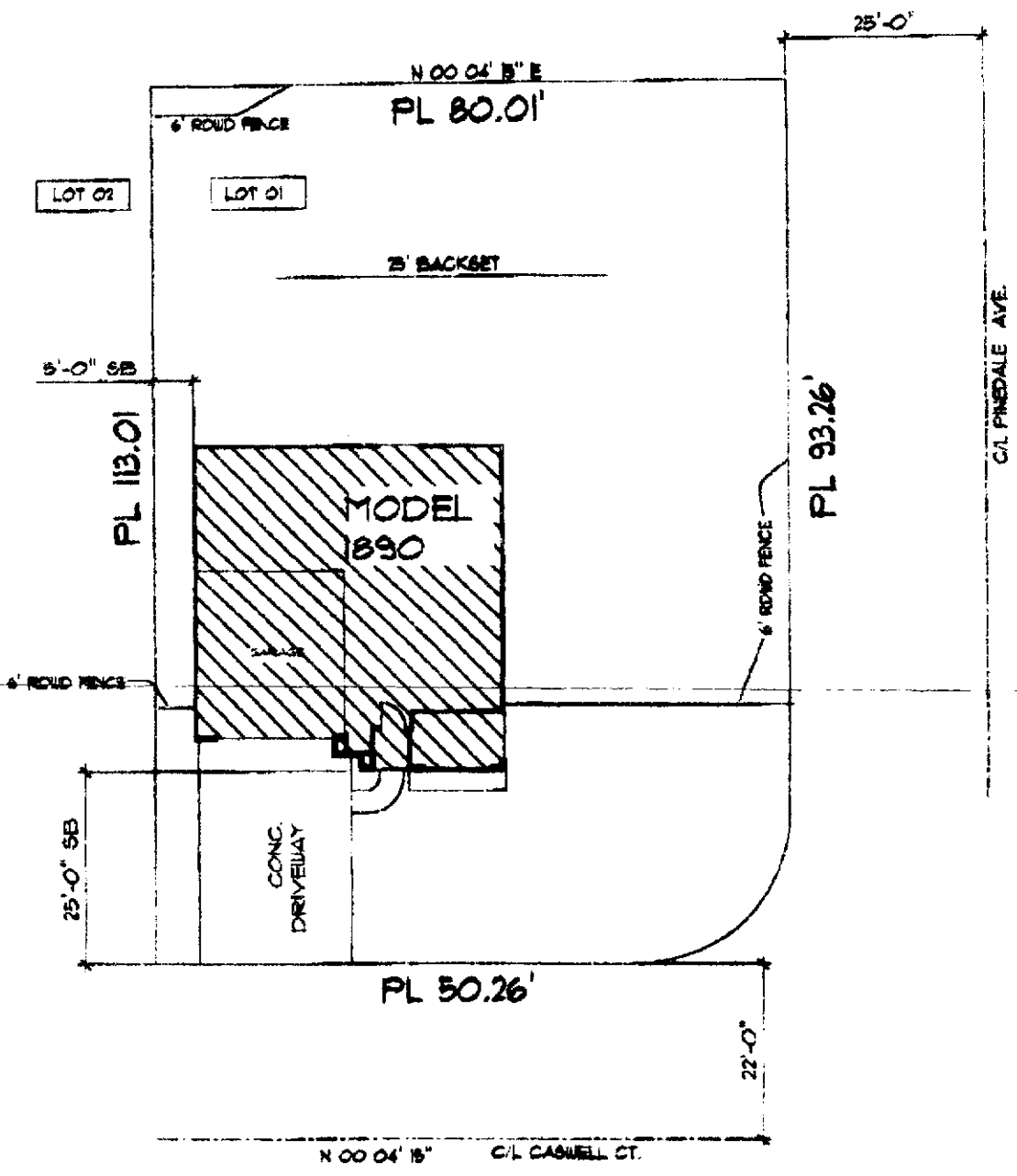
PLOT PLAN LOT 01 SCALE = 1/4" = 1'-0" MOONEY ESTATES
